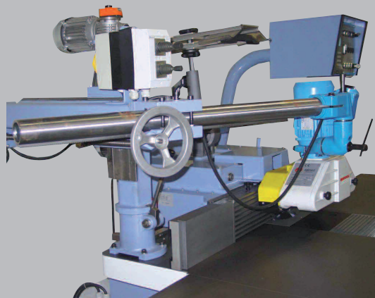
MOTORIZED SUPPORT FOR FEED UNIT
